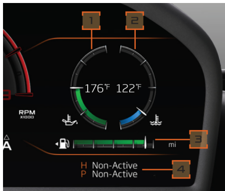
Folding Driver Display - right-hand side
